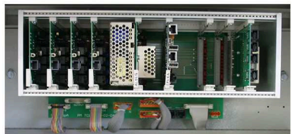
RACK for logic and power supply cards
